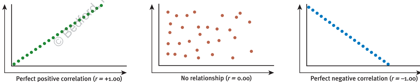
Figure 0.4-1 Scatterplots, showing patterns of correlation
